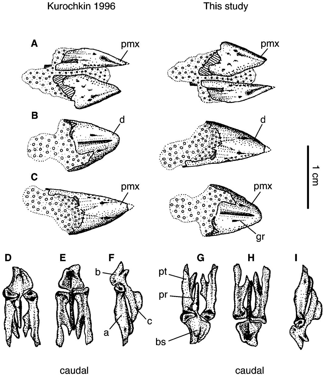
Fig. 5. Skull and mandible of Gobiptyeryx minuta (PIN-4492) as illustrated by Kurochkin (1996) and as interpreted in this study. A , Premaxilla and dentary in lateral view. B , Dentary in ventral view. C , Premaxilla in dorsal view. D–I , Pterygoids, parasphenoid rostrum, and basiptyerygoid in dorsal ( D , G ), ventral ( E , H ), and lateral ( F , I ) views. Modified from Kurochkin (1996: fig. 2). Kurochkin (1996: 10) provided the following with items D , E , and F : paired elements ( a ) rostral portions of pterygoid or pterygoid process of palatine bone; unpaired element ( b ) fused caudal portions of vomers or rostral portions of pterygoids; unpaired element ( c ) rostral portion of parasphenoidal rostrum or nasal septum of mesethmoid. Abbreviations are spelled out in the appendix.
