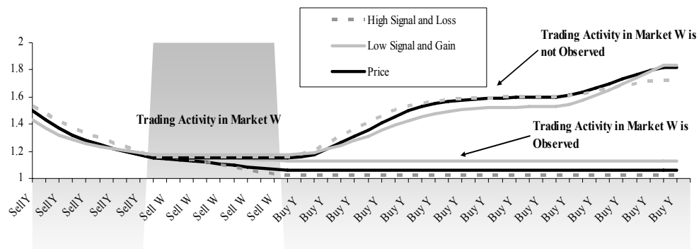
Figure 8. Contagious Spillover in the Case of Independent Asset Values.
