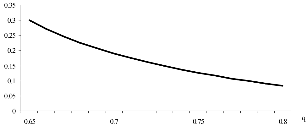
Figure 3. Expected Distance Between the Asymptotic Price and the Fundamental Value.
