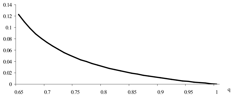
Figure 2. Probability of an Incorrect Cascade.
