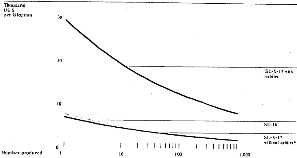
Figure 4 Estimated Cost of Putting a Payload in Near-Earth Orbit With Selected Soviet Launch Vehicles
