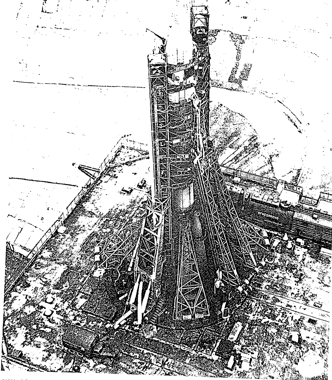
Figure. 4 Soyuz 10 erected on launch pad at Tyuratam
