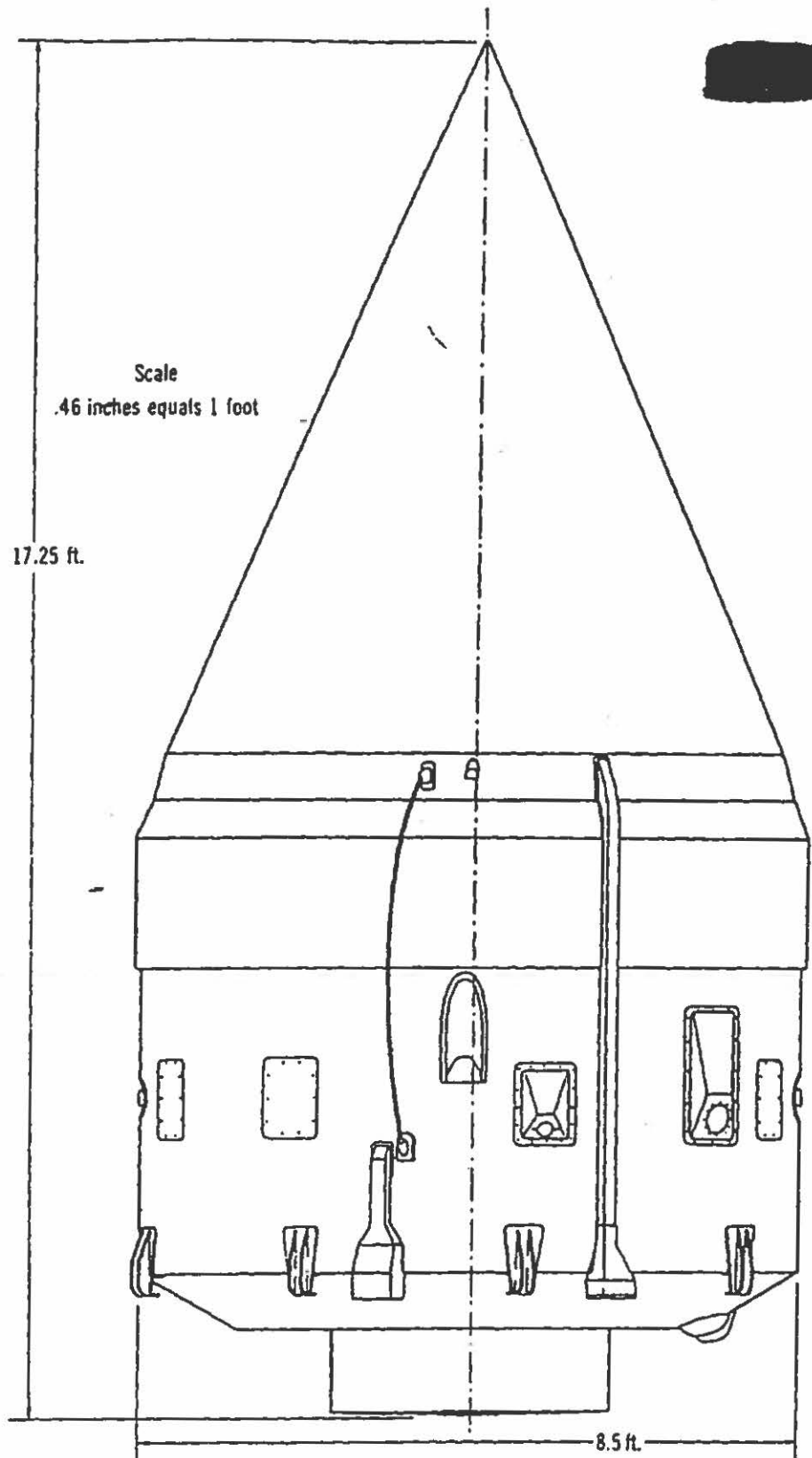
Figure 8. Lunik 1 last stage vehicle, side 2
