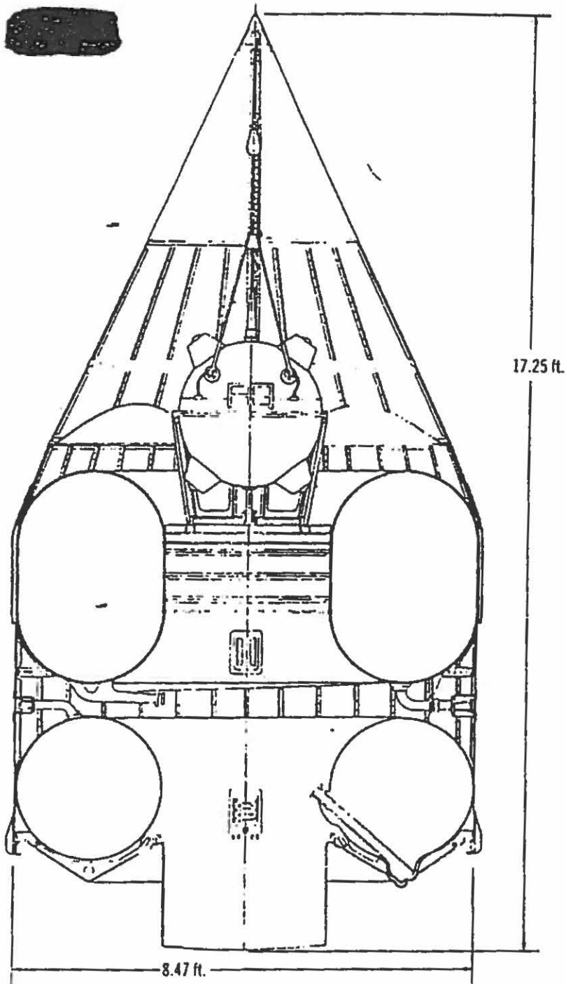
Figure 6. Diagram of Lunik 1 last stage vehicle
