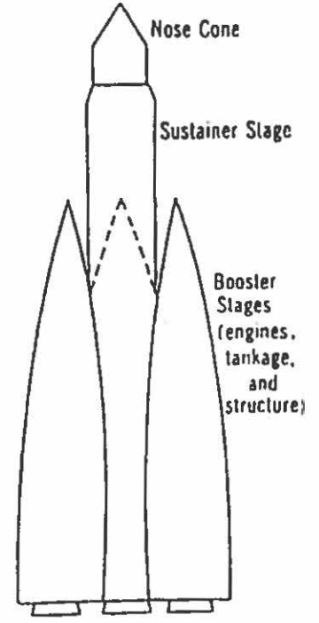
Parallel: All engines fire at launch; booster stages jettisoned prior to sustainer burnout.
