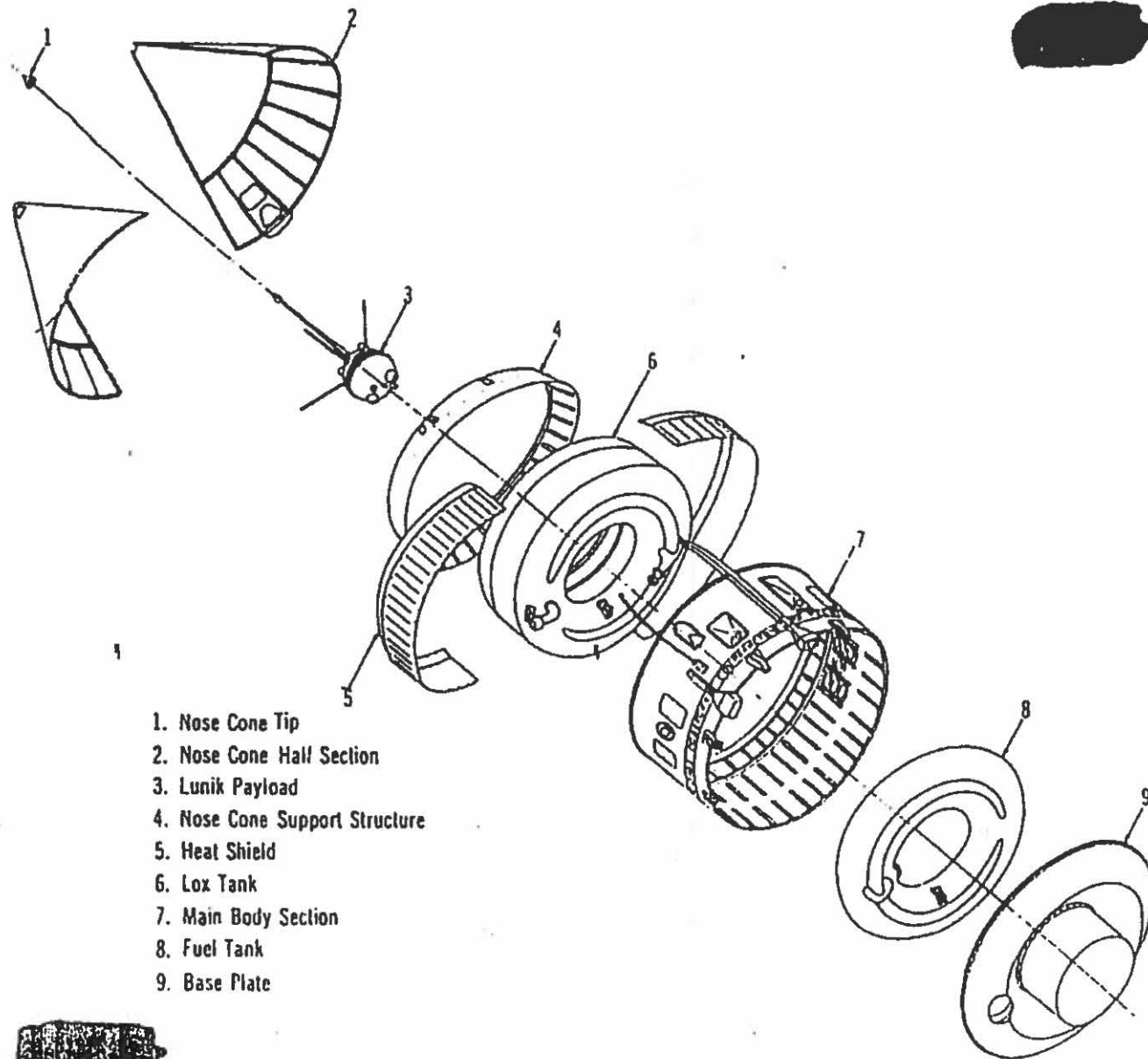
Figure 9. Lunik 1 last stage vehicle, exploded view
