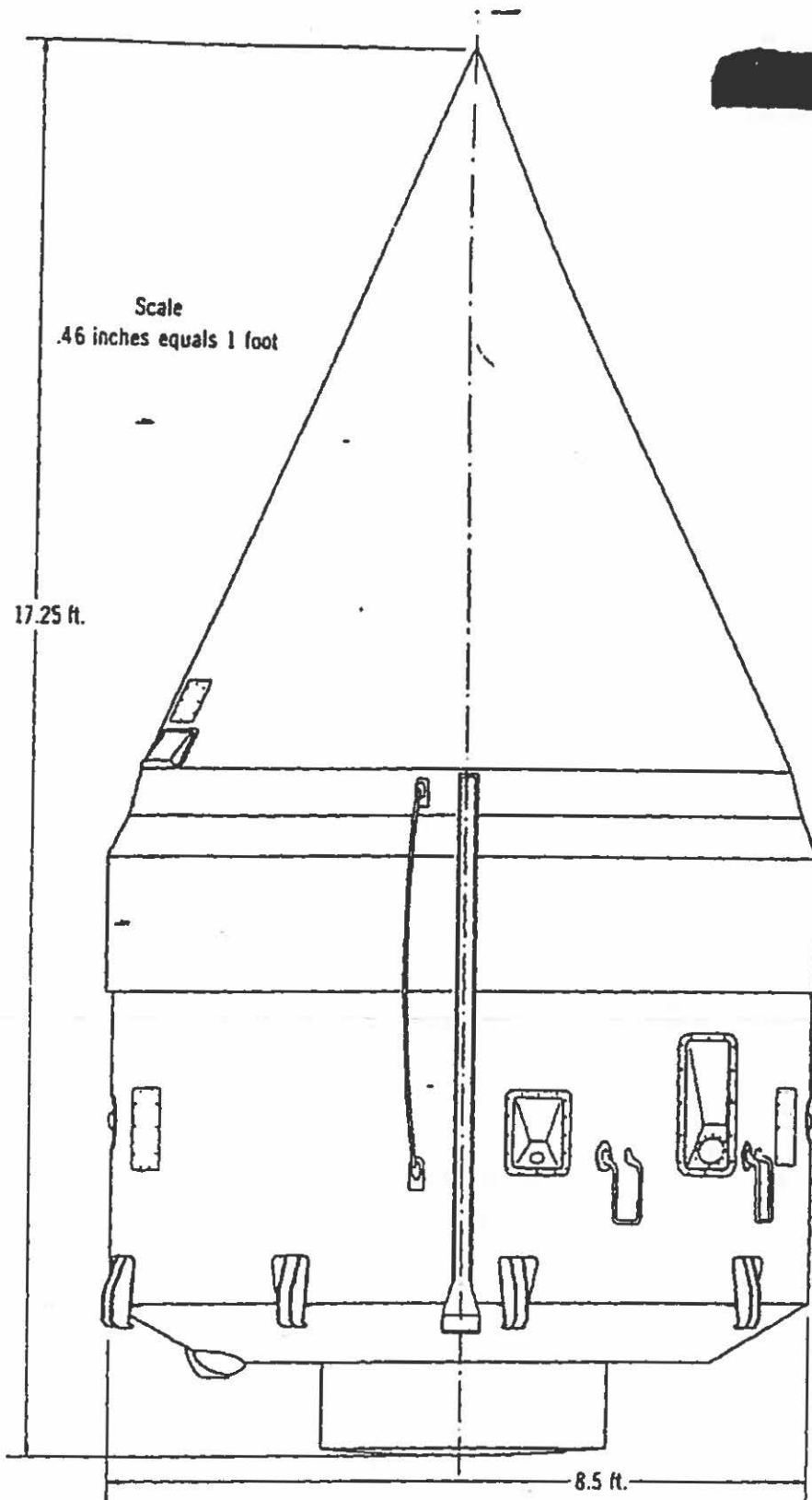
Figure 7. Lunik 1 last stage vehicle, side 1
