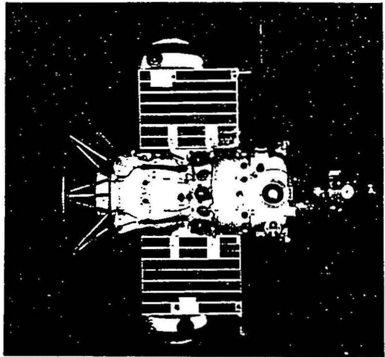
FIGURE 6. Mars 1 Spacecraft.
