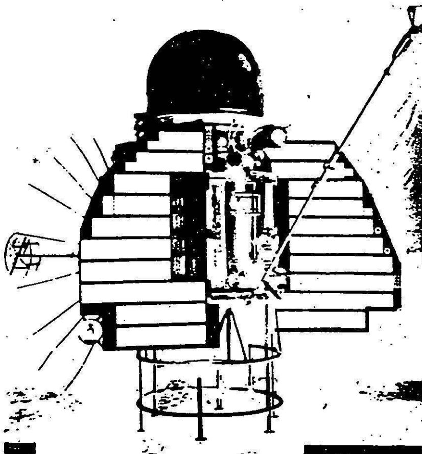
FIGURE 5. Venus 1961 Spacecraft.
