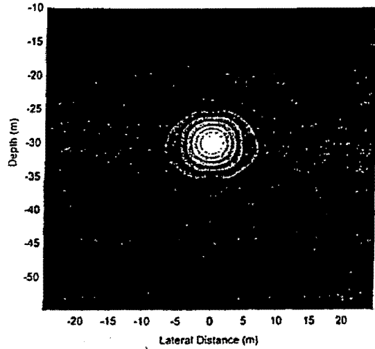
Fig. 3. PSF for a scatterer computed using (16), assuming both surface and borehole data.
