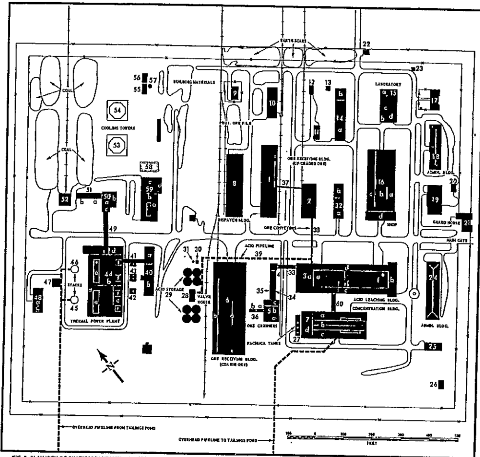
FIG. 8 PLAN VIEW OF PYATIGORSK URANIUM PROCESSING PLANT Note that the perspective view on the opposite page is facing overboard, while the photograph on page 17 is oriented NNE.
