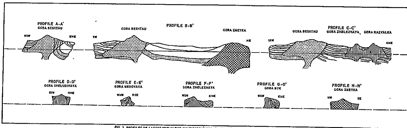
FIG. 3 PROFILES OF LACCOLITHS IN THE PYATIGORSK AREA See Fig. 2 for location and legend for the above profiles
