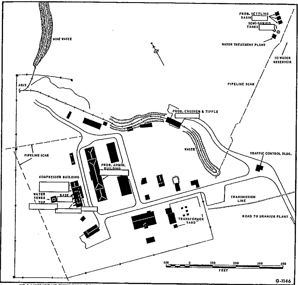
FIG. 5. LARGE MINE AND CRUSHING MILL AT GORA BYK. This small plant processes and up-grades ore from features in the contact zone between igneous and sedimentary deposits.
