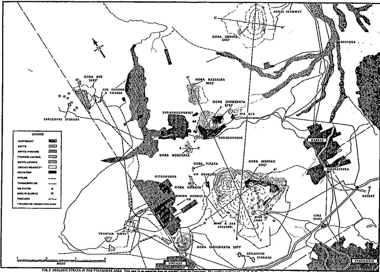
FIG. 2 GEOLOGIC STRATA IN THE PYATIGORSK AREA This map is an adaptation from an original study by Gerasimov. The profiles indicated by A-A', B-B', etc. are shown in cross-section in Figure 1.
