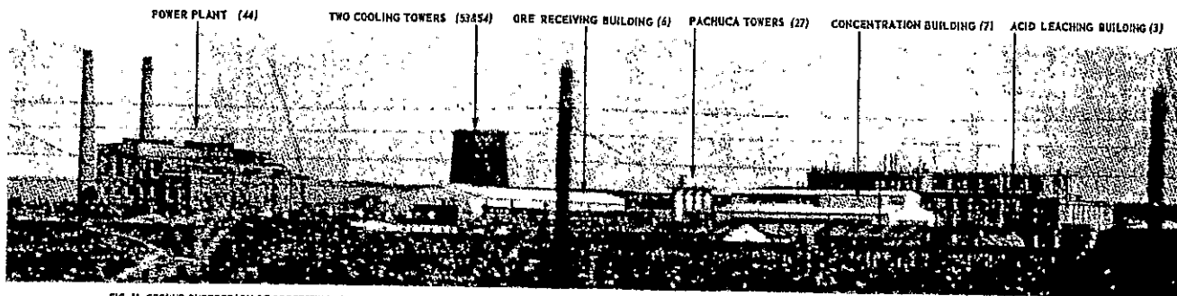
FIG. 11 GROUND PHOTOGRAPH OF PROCESSING PLANT. Photograph taken from highway southwest of plant on 20 Nov. 1956. Numbers refer to building location in Fig. 8. Note presence of only one cooling tower [redacted]
